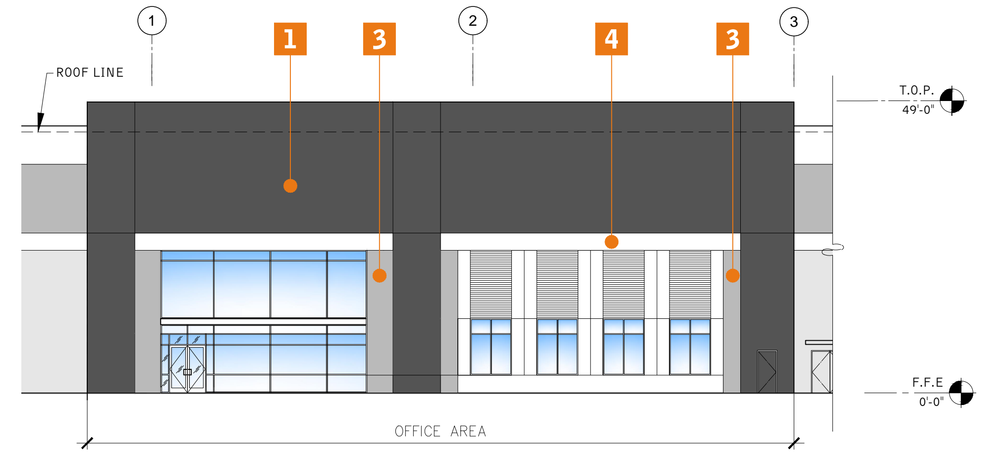
ENLARGED SOUTH ELEVATION - CENTER OFFICE AREA | 2 1/16" = 1'-0"
