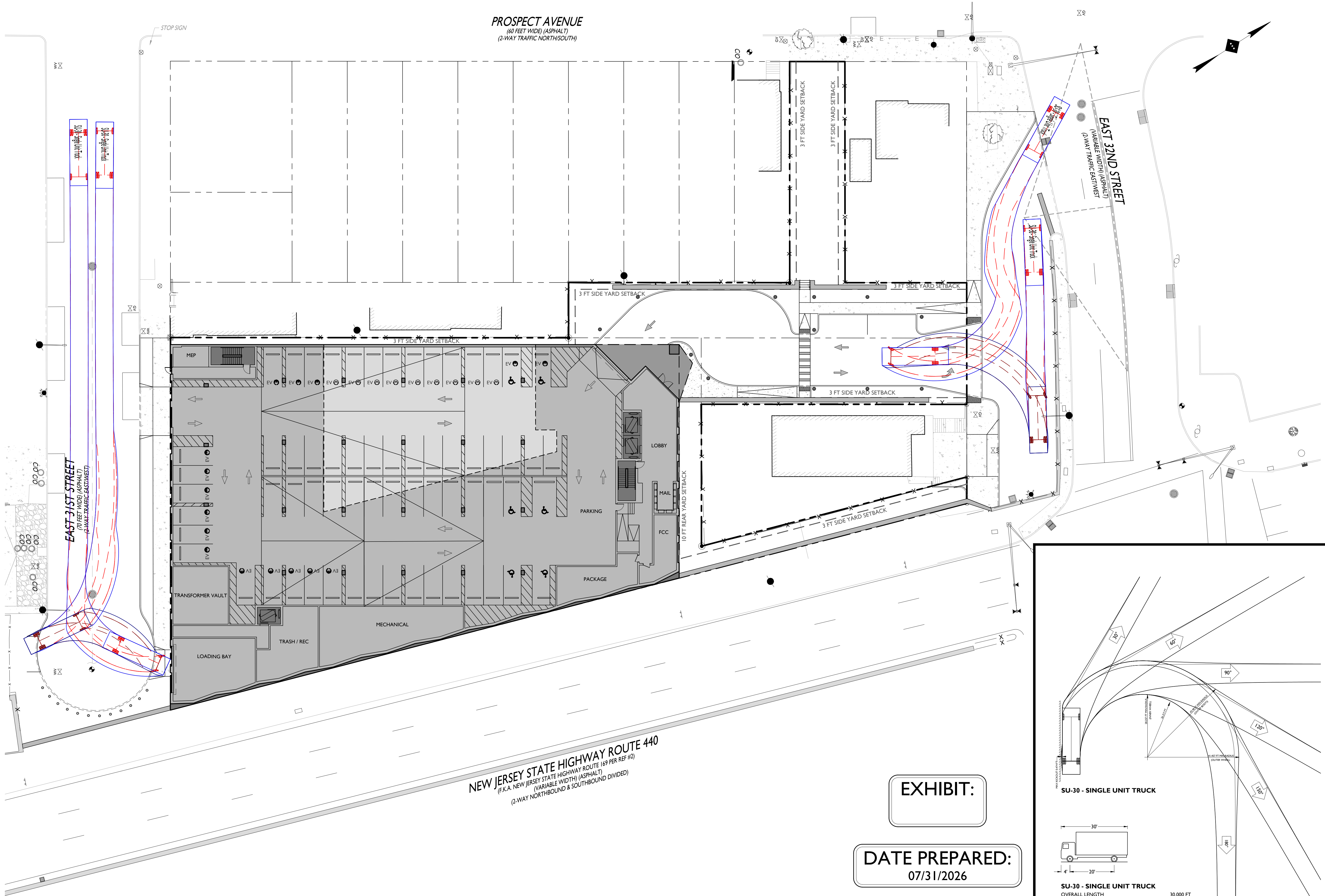
SU-30 - SINGLE UNIT TRUCK
