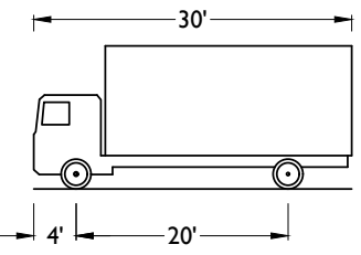
SU-30 - SINGLE UNIT TRUCK
