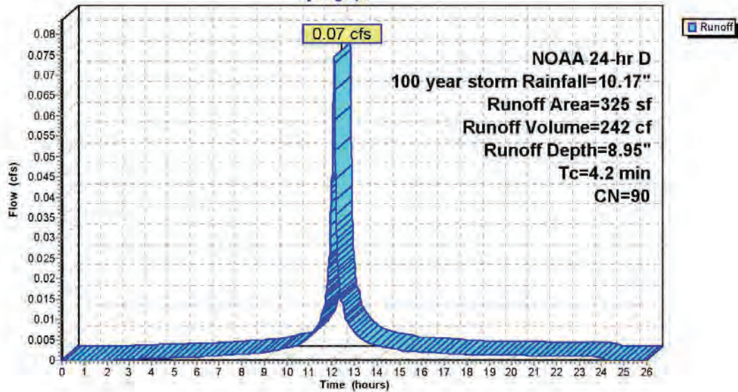
Hydrograph
