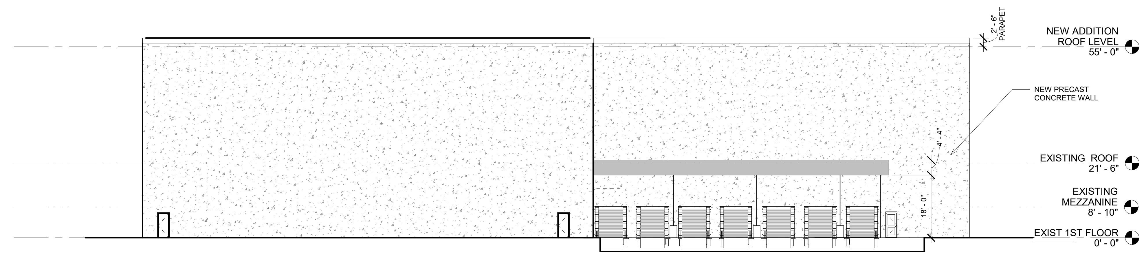
3 NORTH ELEVATION 1/16" = 1'-0"
